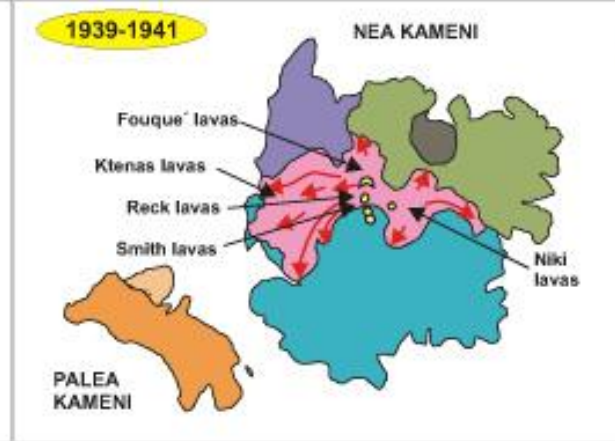
THE CREATION OF PALEA AND NEA KAMENI Institute for the Study and Monitoring of the Santorini Volcano
